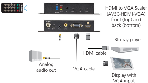
Figure 3-1. Typical application.
