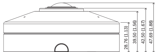
Dimensions in mm (in.)
